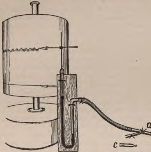
FIG. 48.—The modern method of measuring blood-pressure in animals. A glass nozzle or cannula like ( c ) is tied into an artery as at ( a ). The pressure elevates the more distant limb of a mercury column in a U-tube and a float on the mercury causes a writing-point to trace upon a revolving drum. Transmission from the blood to the mercury is by tubing filled with a solution restraining coagulation.
